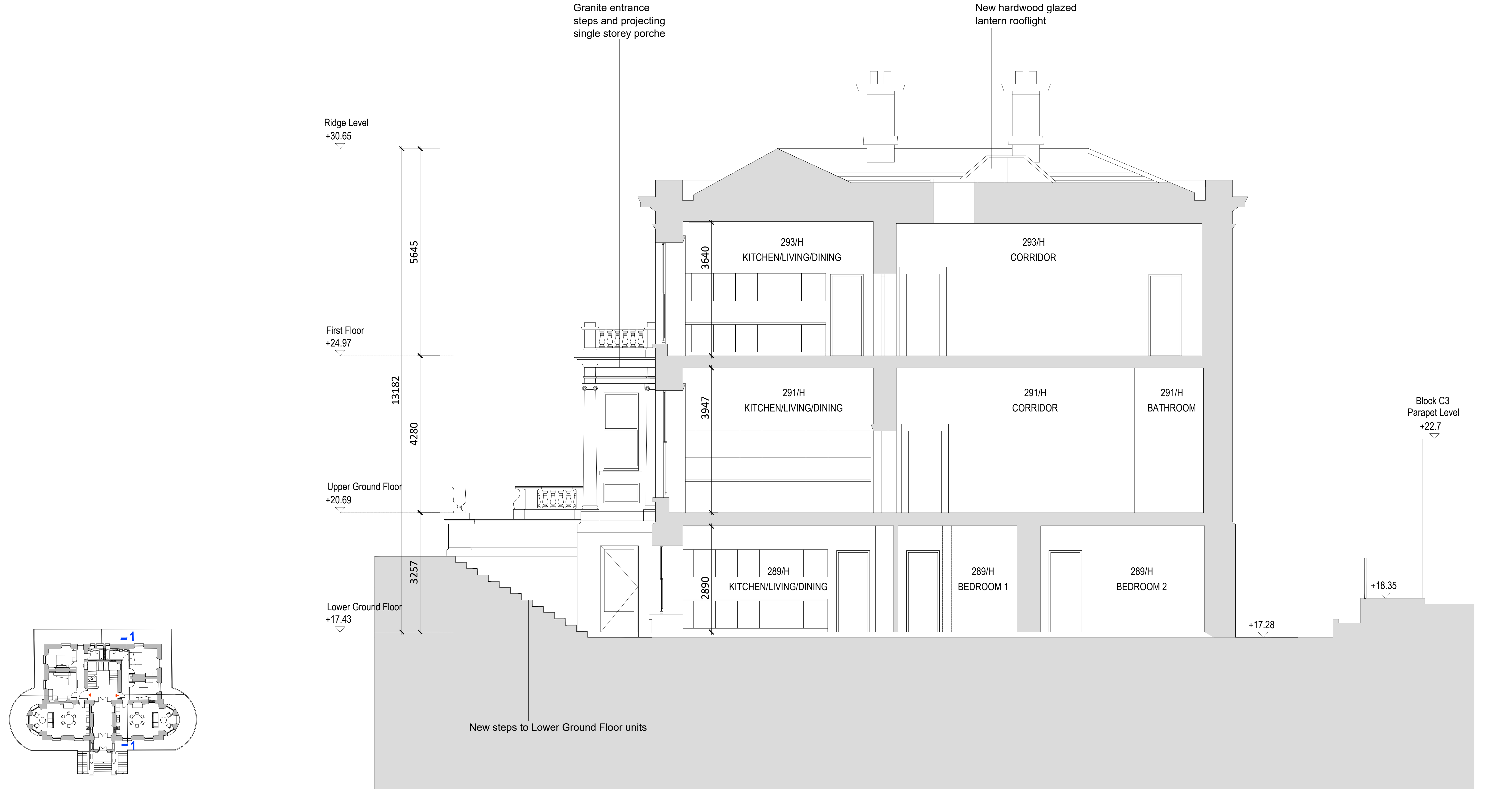
PROPOSED SECTION 1-1 - St. Teresa's House
